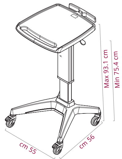
WORK PLANE
